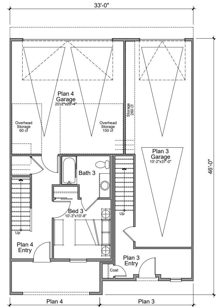
Plan 4 First Floor 341 Net SQ. FT.
