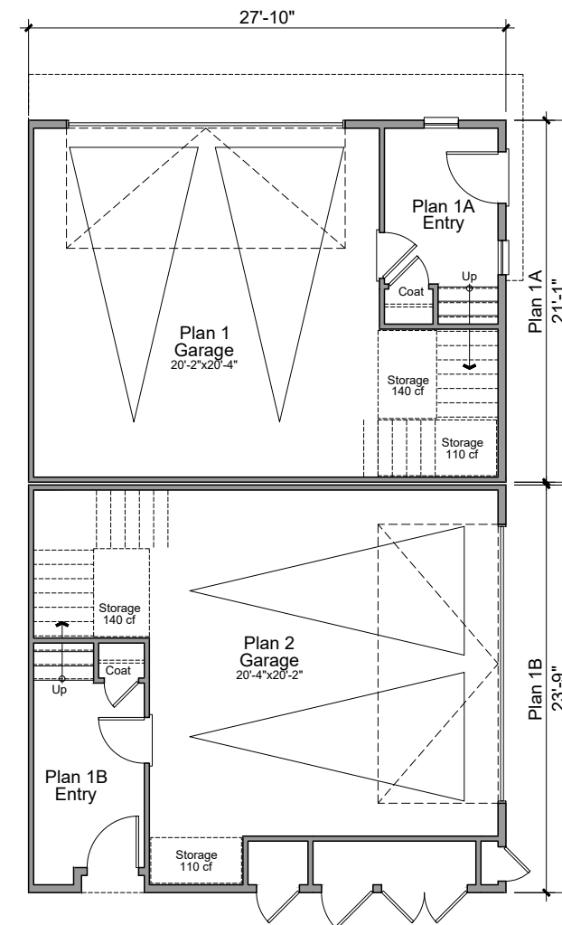
Plan 1B First Floor 137 Net SQ. FT.
