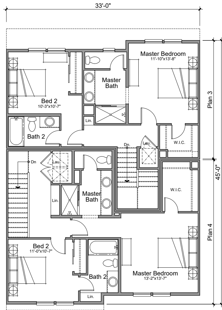
Plan 4 Third Floor 666 Net SQ. FT.
