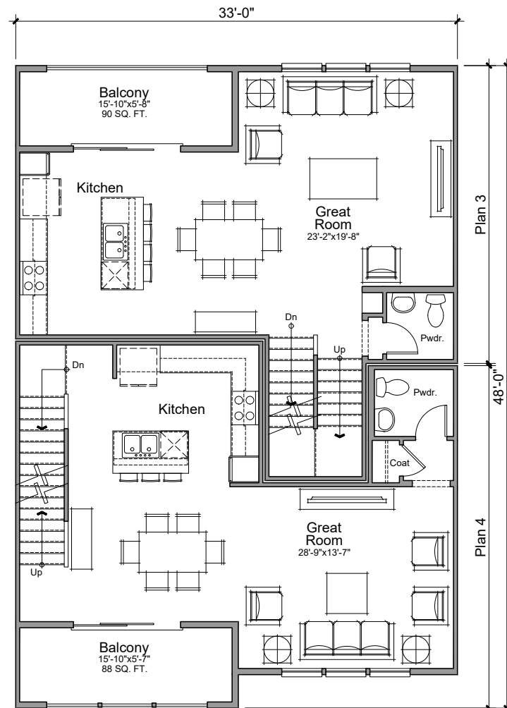
Plan 4 Second Floor 625 Net SQ. FT.
